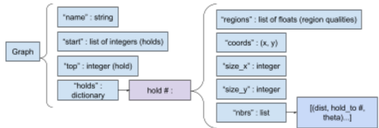
Figure 3: Graph Structure
